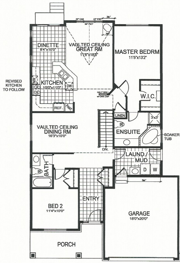
Ground Floor (1,500 sq.ft.)
